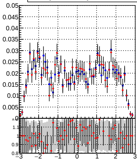
DQM_TT_mkFit-DQM_original DQM_TT_mkFit-DQM_modified4
