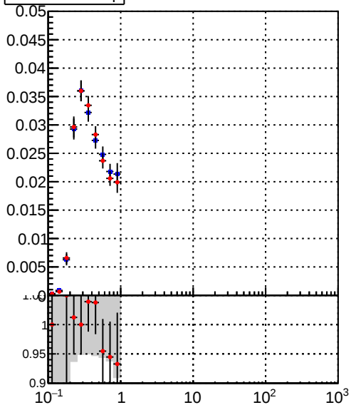
DQM_TT_mkFit-DQM_original DQM_TT_mkFit-DQM_modified4
