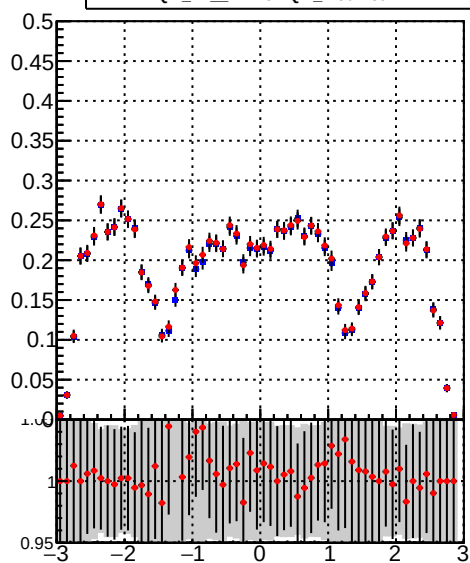
—■— DQM_TT_mkFit-DQM_original —●— DQM_TT_mkFit-DQM_modified4
