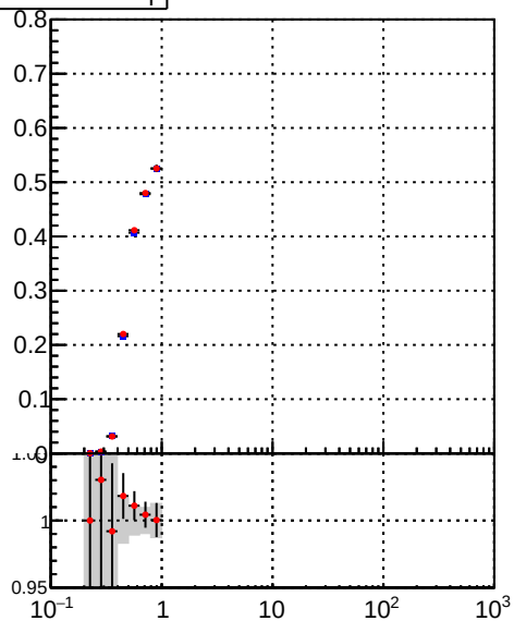
—■— DQM_TT_mkFit-DQM_original —●— DQM_TT_mkFit-DQM_modified4
