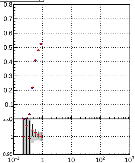
— DQM_TT_mkFit-DQM_original — DQM_TT_mkFit-DQM_modified4
