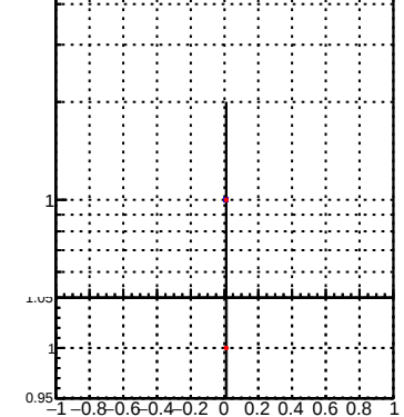
N of associated tracks (simToReco) vs dz(PV)
