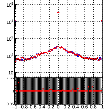
N of simulated tracks vs dz(PV)
