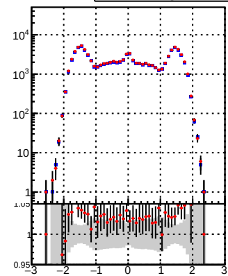
—●— DQM_TT_mkFit-DQM_original —●— DQM_TT_mkFit-DQM_modified4
