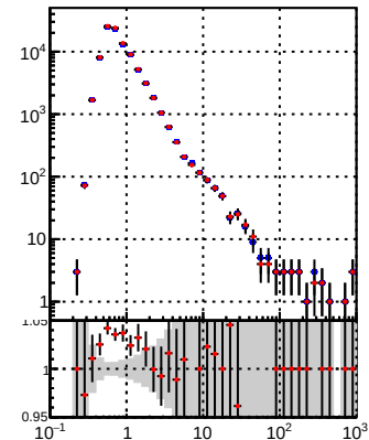
—●— DQM_TT_mkFit-DQM_original —●— DQM_TT_mkFit-DQM_modified4
