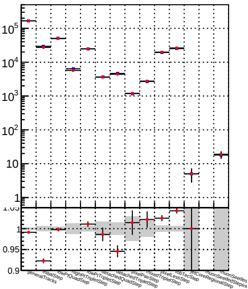
Number —●— DQM_TT__mkFit-DQM_modified4
