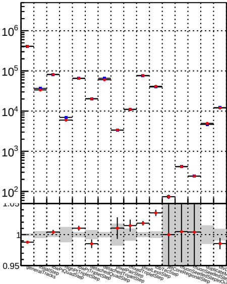
Number —●— DQM_TT__mkFit-DQM_modified4
