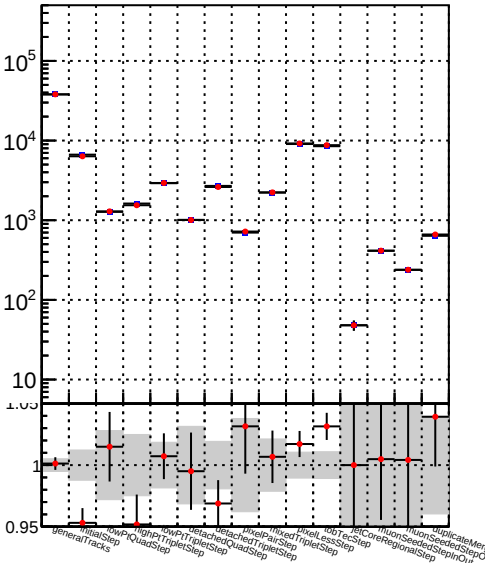
Number —●— DQM_TT_mkFit-DQM_modified4
