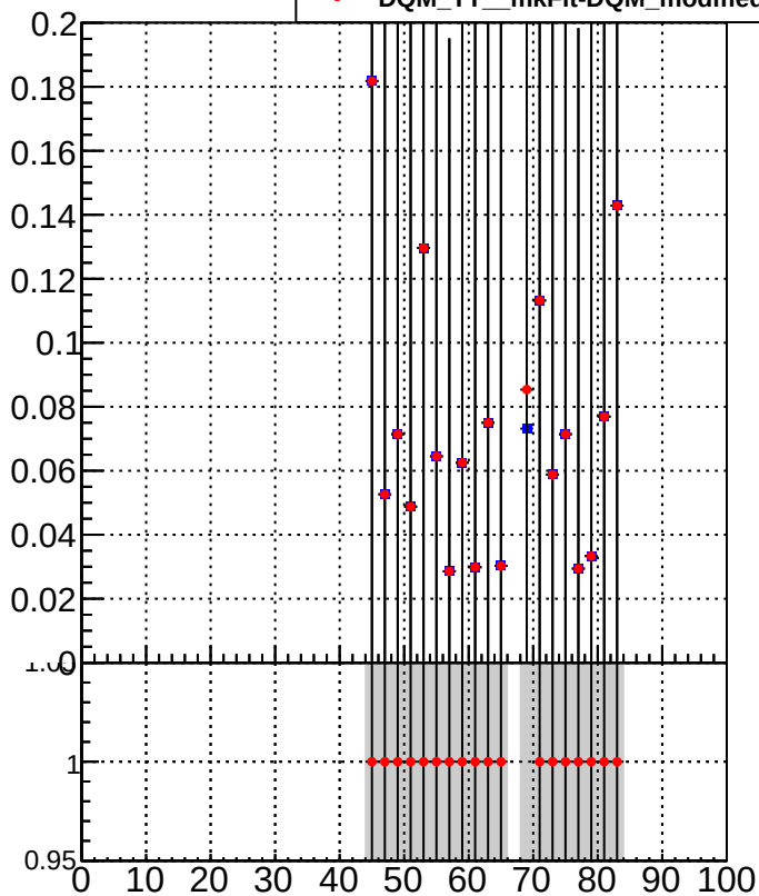
—■— DQM_TT_mkFit-DQM_original —●— DQM_TT_mkFit-DQM_modified4
