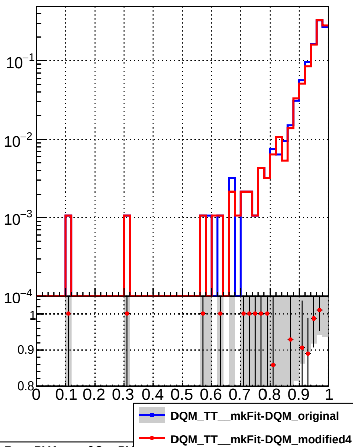
RecoPVAssoc2GenPVMatched_Missing
