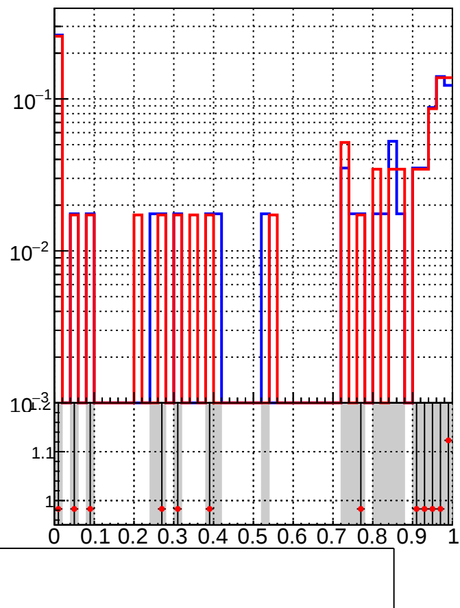
RecoPVAssoc2GenPVNotMatched_Missing
