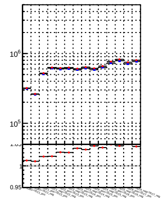
N of reco track vs. \chi^2 mkFit-DQM_original mkFit-DQM_modified4
