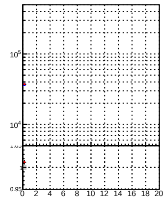
Legend: DQM TT mkFit-DQM_original (blue line), DQM TT mkFit-DQM_modified4 (red line), verSet (grey shaded area)
