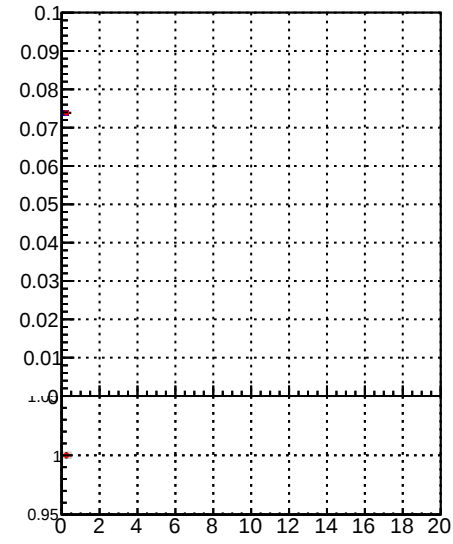
Fake rate vs. — \bullet DQM TT mkFit-DQM_original — \bullet DQM TT mkFit-DQM_modified4
