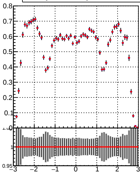
— DQM_TT_mkFit-DQM_original — DQM_TT_mkFit-DQM_modified4
