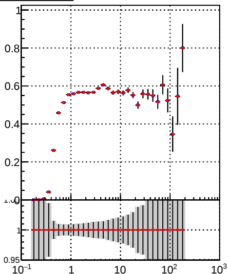
— DQM_TT_mkFit-DQM_original — DQM_TT_mkFit-DQM_modified4
