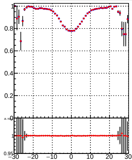
—•— DQM_TT_mkFit-DQM_original —•— DQM_TT_mkFit-DQM_modified4
