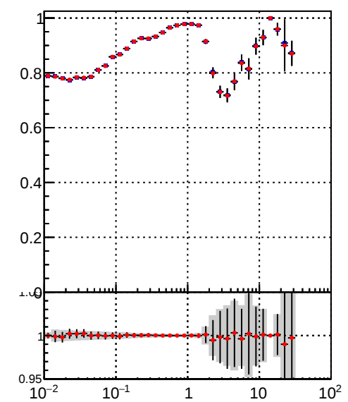
Efficiency vs vertpos — DQM_TT_mkFit-DQM_original — DQM_TT_mkFit-DQM_modified4
