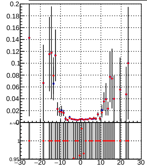
Efficiency vs vertpos — DQM_TT_mkFit-DQM_original — DQM_TT_mkFit-DQM_modified4
