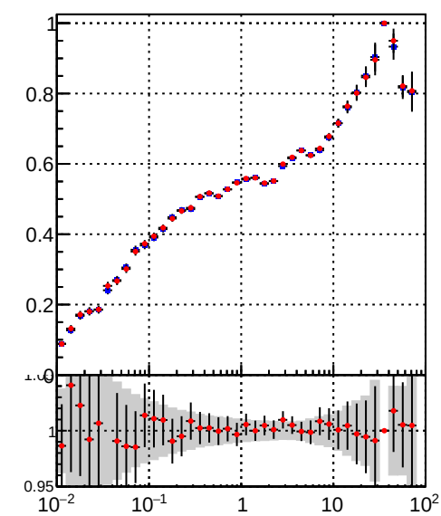
Efficiency vs. sim PV z Legend: DQM_TT_mkFit-DQM_original (blue) DQM_TT_mkFit-DQM_modified4 (red)
