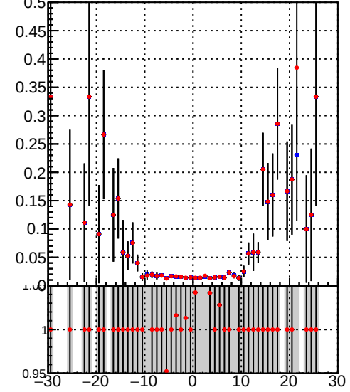
Efficiency vs. sim PV z Legend: DQM_TT_mkFit-DQM_original (blue) DQM_TT_mkFit-DQM_modified4 (red)
