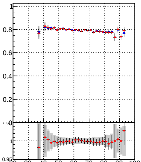
Efficiency vs NumVertices
