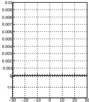
Duplicates Rate vs Dz(PV)
