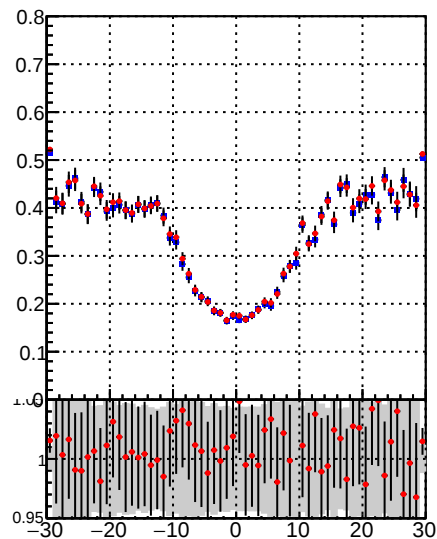
—•— DQM_TT_mkFit-DQM_original —•— DQM_TT_mkFit-DQM_modified4
