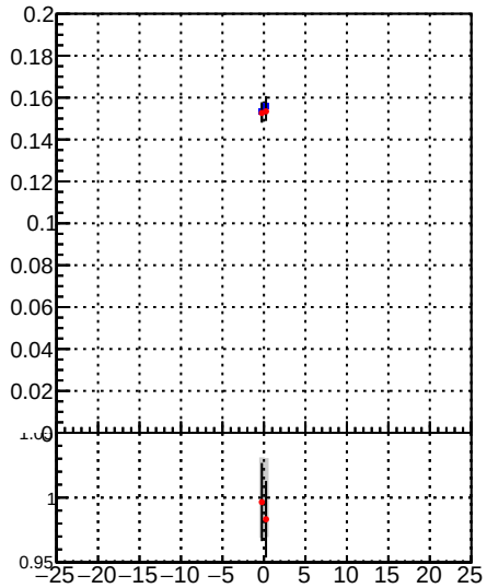
Fake rate vs d Legend: - Blue line with dots: DQM TT mkFit-DQM_original - Red line with dots: DQM TT mkFit-DQM_modified4
