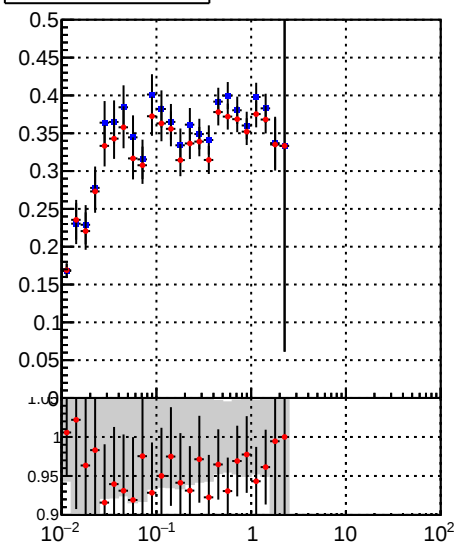
—•— DQM_TT_mkFit-DQM_original —•— DQM_TT_mkFit-DQM_modified4
