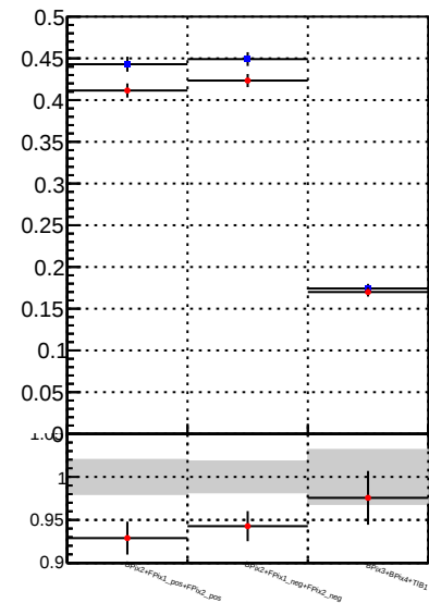
Fake rate vs. —●— DQM_TT_mkFit-DQM_original —●— DQM_TT_mkFit-DQM_modified4
