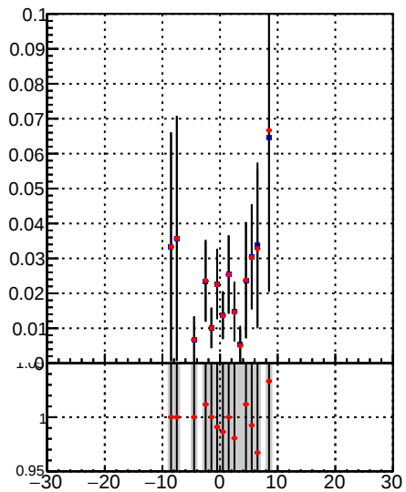
—●— DQM_TT_mkFit-DQM_original —●— DQM_TT_mkFit-DQM_modified4
