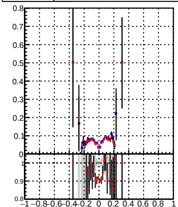
—●— DQM_TT_mkFit-DQM_original —●— DQM_TT_mkFit-DQM_modified4
