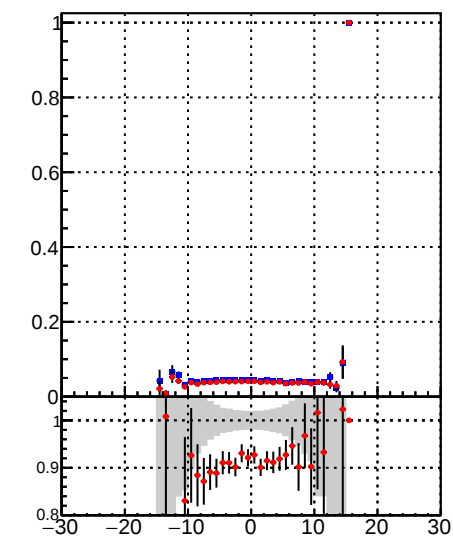
Fake rate vs d DQM_TT_mkFit-DQM_original DQM_TT_mkFit-DQM_modified4
