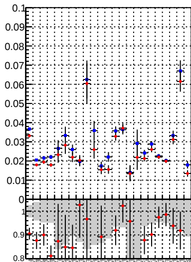
Fake rate vs. —•— DQM_TT_mkFit-DQM_original —•— DQM_TT_mkFit-DQM_modified4
