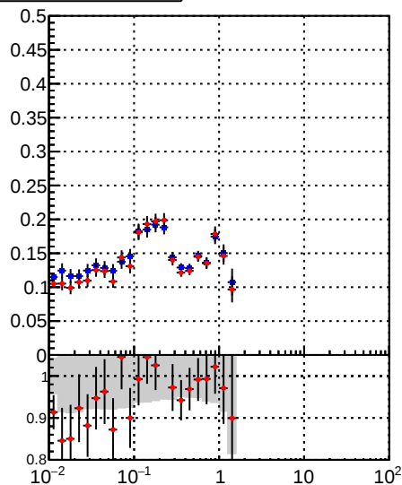
—•— DQM_TT_mkFit-DQM_original —•— DQM_TT_mkFit-DQM_modified4
