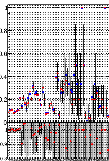
Fake rate vs. —•— DQM_TT_mkFit-DQM_original —•— DQM_TT_mkFit-DQM_modified4
