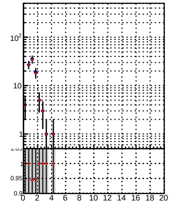
N of reco track vs. \chi^2 DQM TT mkFit-DQM_original DQM TT mkFit-DQM_modified4
