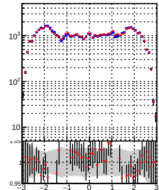
—●— DQM_TT_mkFit-DQM_original —●— DQM_TT_mkFit-DQM_modified4
