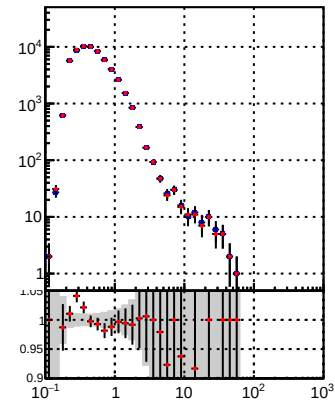
—●— DQM_TT_mkFit-DQM_original —●— DQM_TT_mkFit-DQM_modified4
