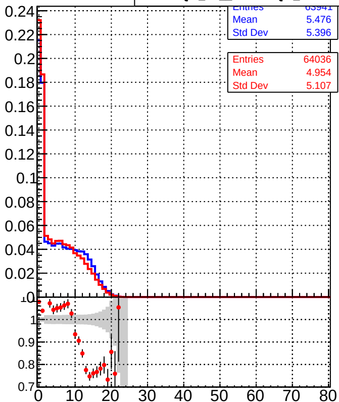
■ DQM_TT_mkFit-DQM_original ● DQM_TT_mkFit-DQM_modified4
