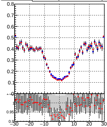
—•— DQM_TT_mkFit-DQM_original —•— DQM_TT_mkFit-DQM_modified4
