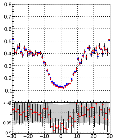
Fake rate vs d —●— DQM_TT_mkFit-DQM_original —●— DQM_TT_mkFit-DQM_modified4
