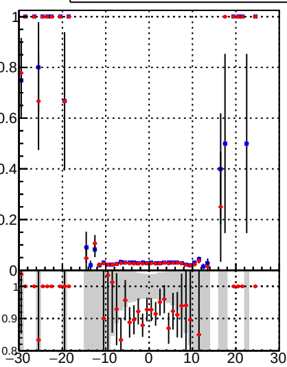
—●— DQM_TT_mkFit-DQM_original —●— DQM_TT_mkFit-DQM_modified4
