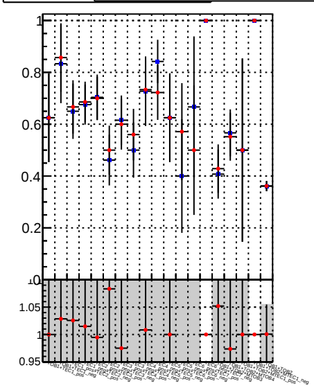
Fake rate vs. — DQM_TT_mkFit-DQM_original — DQM_TT_mkFit-DQM_modified4
