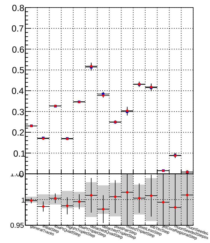
Duplicates rate vs collection Legend: DQM_TT_mkFit-DQM_original (Blue square) DQM_TT_mkFit-DQM_modified4 (Red circle)
