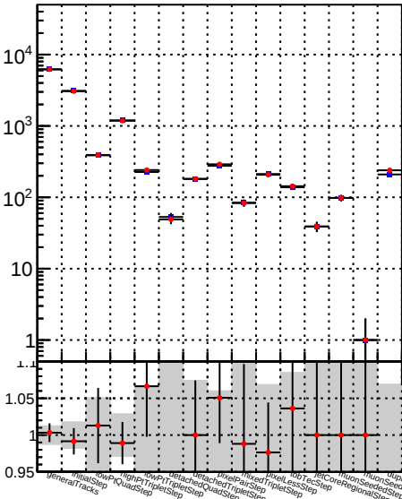
Number —●— DQM_TT_mkFit-DQM_modified4
