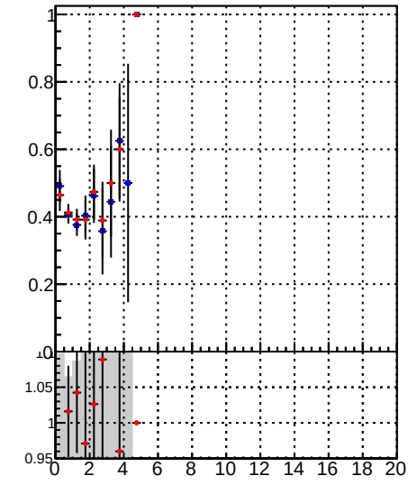
Fake rate vs. —●— DQM_TT_mkFit-DQM_original —●— DQM_TT_mkFit-DQM_modified4
