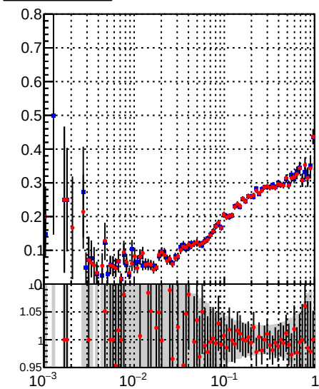
Fake rate vs \mu DQM_TT_mkFit-DQM_original DQM_TT_mkFit-DQM_modified4
