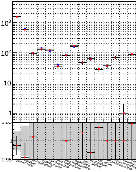
Number —●— DQM_TT_mkFit-DQM_modified4
