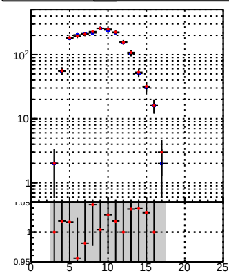
DQM_TT_mkFit-QM_original DQM_TT_mkFit-QM_modified4
