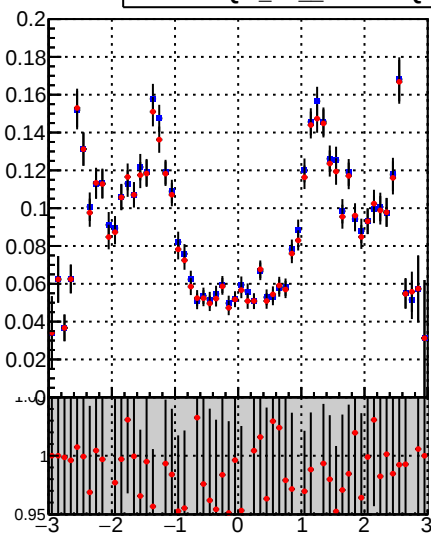
—■— DQM_TT_mkFit-DQM_original —●— DQM_TT_mkFit-DQM_modified4
