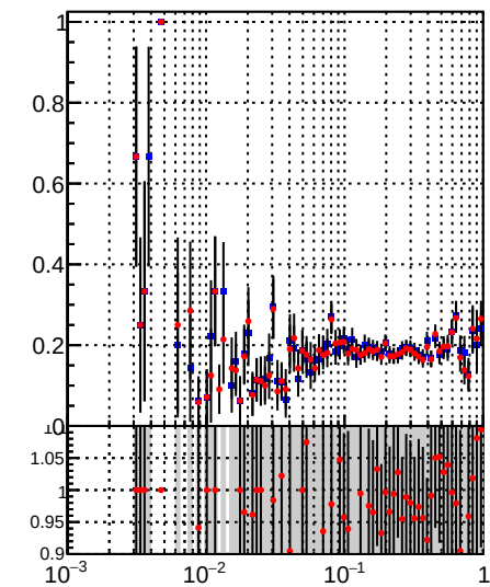
■ DQM_TT_mkFit-DQM_original ● DQM_TT_mkFit-DQM_modified4
