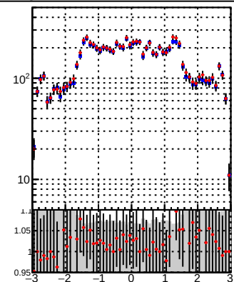
—●— DQM_TT_mkFit-DQM_original —●— DQM_TT_mkFit-DQM_modified4
