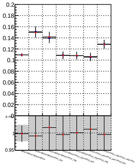
Fake rate vs. —●— DQM TT mkFit-DQM_original —●— DQM TT mkFit-DQM_modified4
