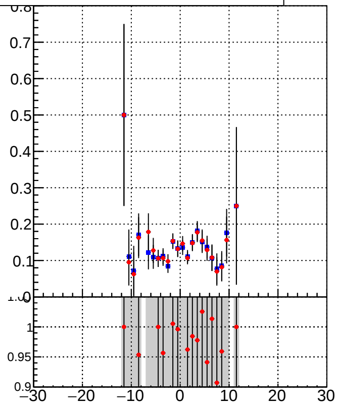
DQM_TT_mkFit-DQM_original DQM_TT_mkFit-DQM_modified4
