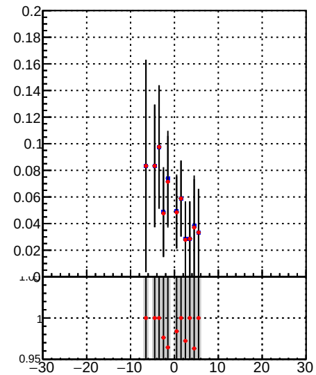
Fake rate vs d —●— DQM TT mkFit-DQM_original —●— DQM TT mkFit-DQM_modified4
