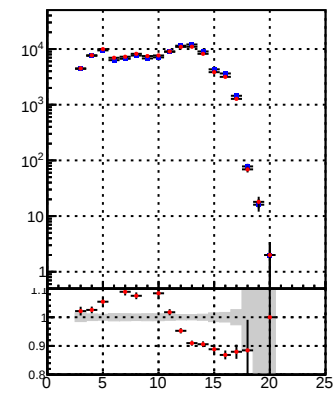
—•— DQM_TT_mkFit-DQM_original —+— DQM_TT_mkFit-DQM_modified4
