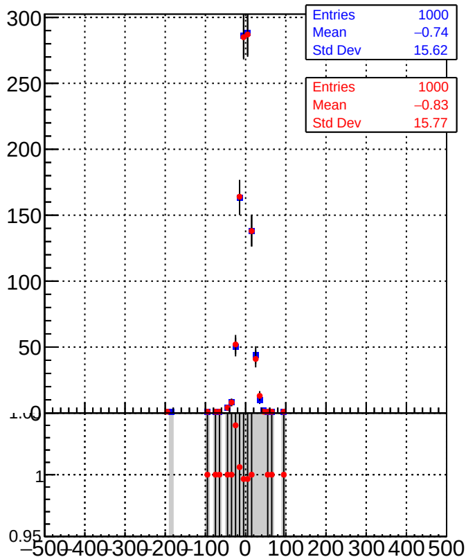
Y distance from BeamSpot (tagged Vtx)
